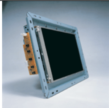
KEYTEC'S Magic Touch integrated on 6.4" open frame LCD
